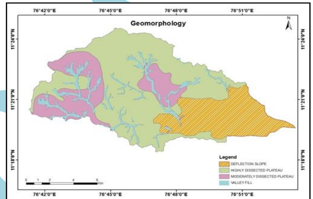
Fig.8. Geomorphology map of the watersheds
