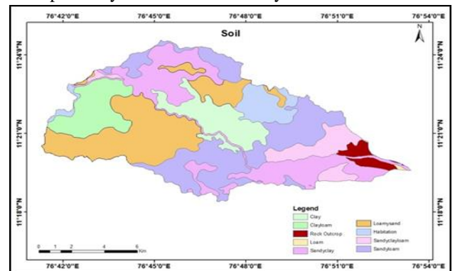
Fig.9.soil map of the watershed
