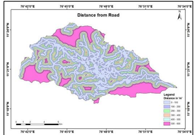
Fig.11. Distance to Road Map of the Watersheds
