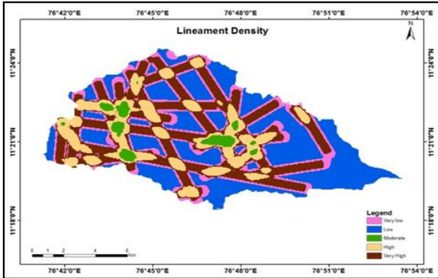
Fig.6 .Lineament density map of the study area
