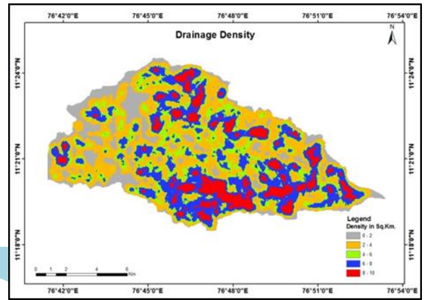
Fig.4 .Drainage map of the study area
