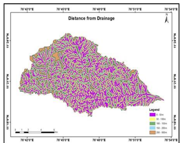
Fig 5 Distance to Drainage map of the study area
