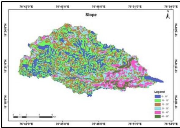
Fig.2.Slope map of the watersheds
