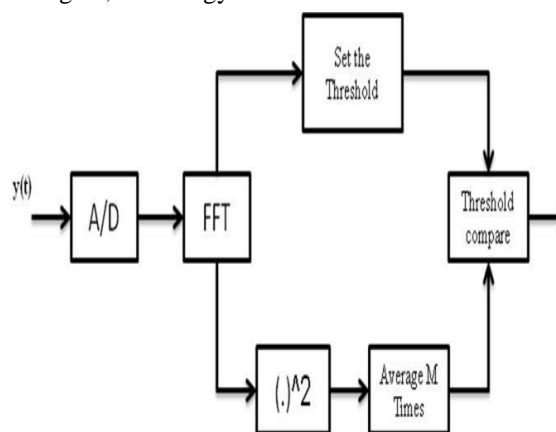
Fig.2 Digital implementation of an energy detector
