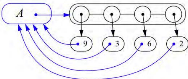
Figure 2: Representation of partition
