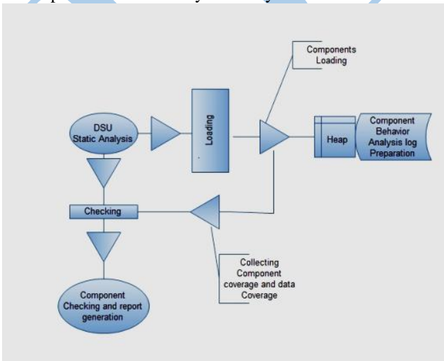
Fig 1 Architecture of the proposed framework
