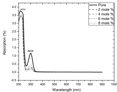
Fig7. UV – Vis – NIR spectrum of pure and doped GSN
