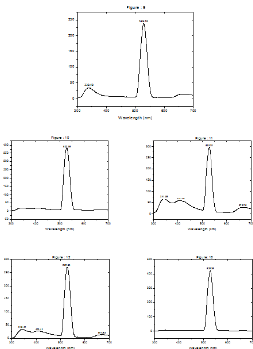
Fig. 9-13.PL spectra of Pure, 2,4,6 and 8 mole % doped GSN crystals respectively
