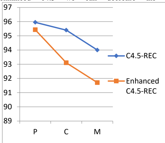
Fig -3 Recall (REC) C4.5&Enhanced C4.5
