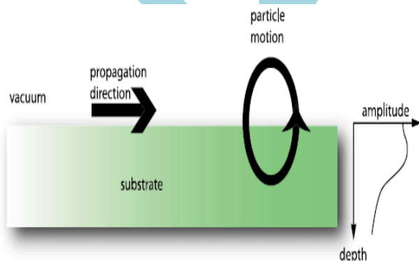
Fig 1. Basic Surface Acoustic Wave
